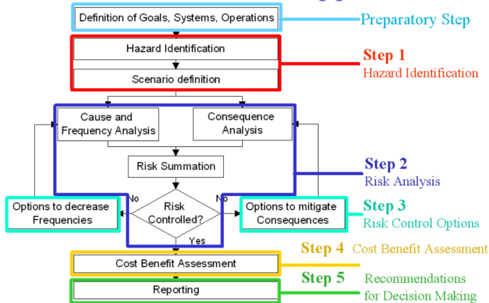
Fig. 1 FSA Flowchart [IACS – MSC 75, 2002]
