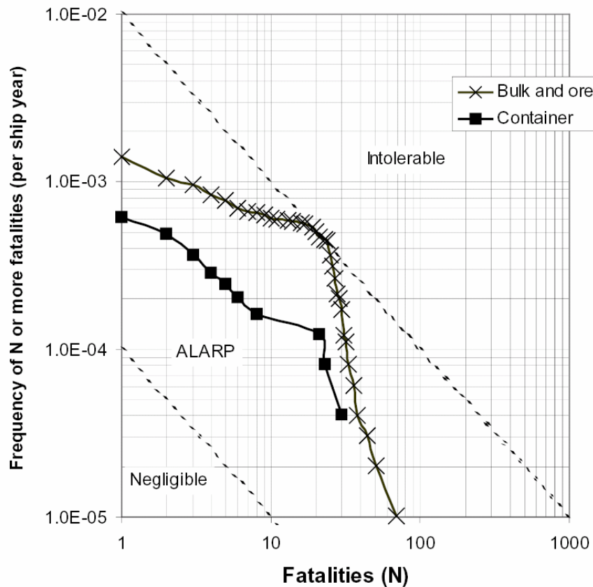
Fig 6 F-N Diagram (crew) [Skjong and Eknes, 2001]
