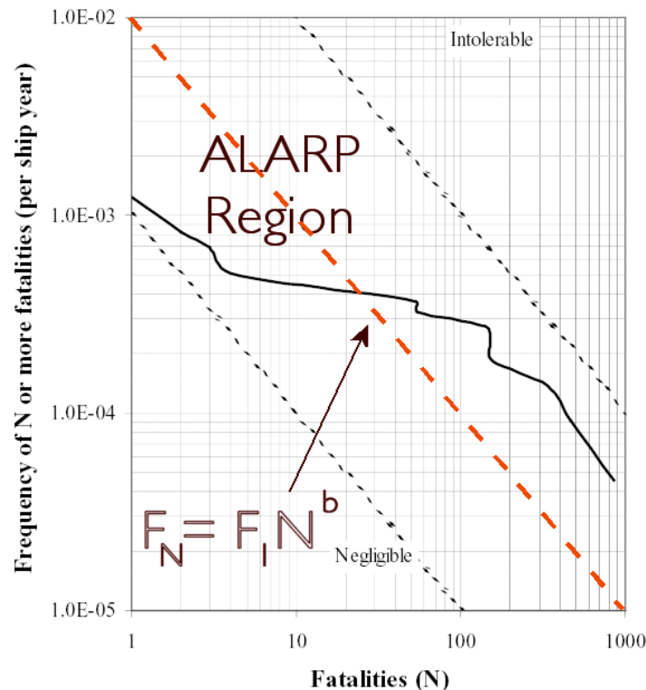
Fig 4 Typical F-N Diagram
