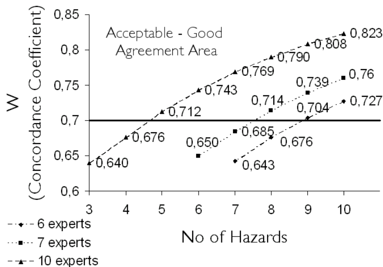
Fig. 2 Concordance Coefficient in one “extreme swap” [Kontovas, 2005]
