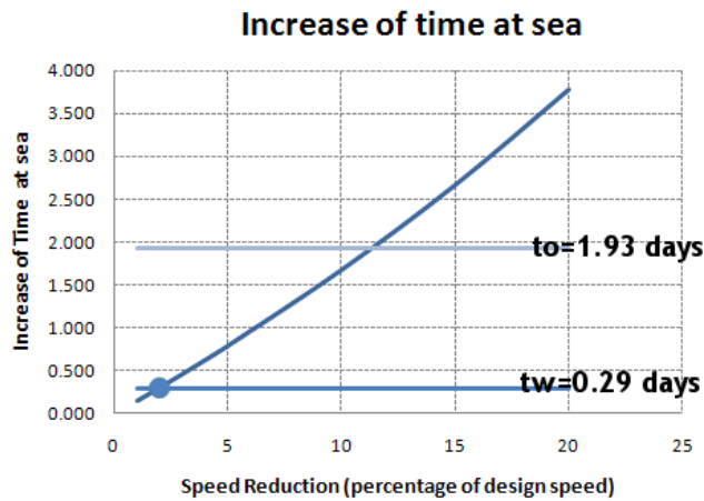
Fig. 5: Time implications of speed reduction
