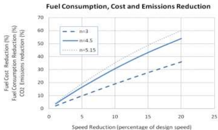
Fig. 4: Reduction percentage due to speed reduction
