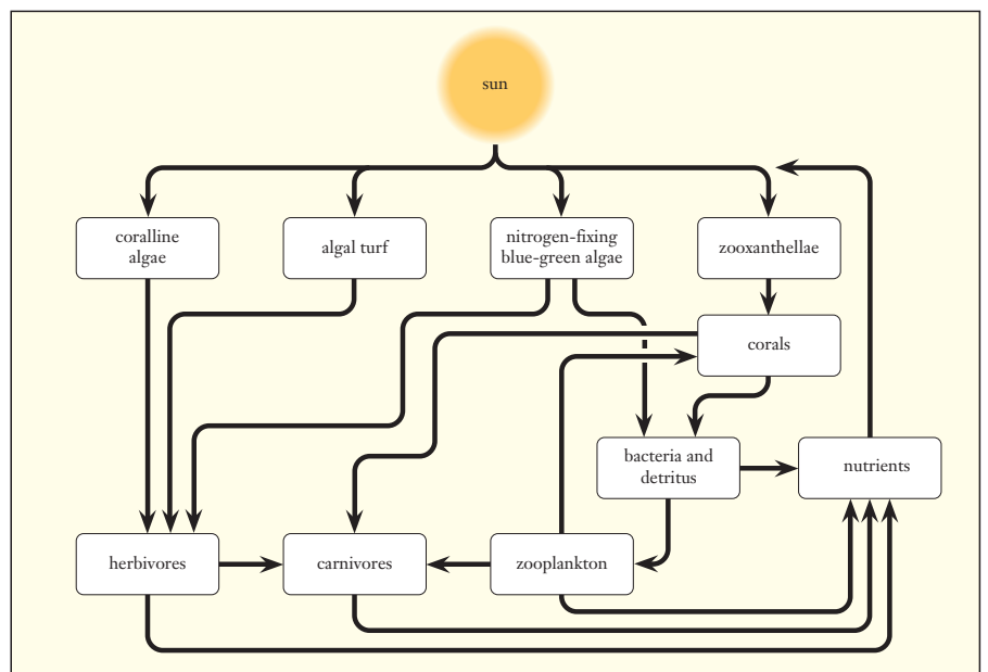
Right: A simplified diagram of how a reef ecosystem works, with the zooxanthellae interacting with the coral, the coralline algae which cement the structure, and the filamentous blue-green algae (cyanobacteria) providing much of the nitrogen fixation. The algae are eaten by the herbivores which in turn are a food source for the carnivores, as are the zooplankton. The cycles are completed by the release of nutrients back into the system.
