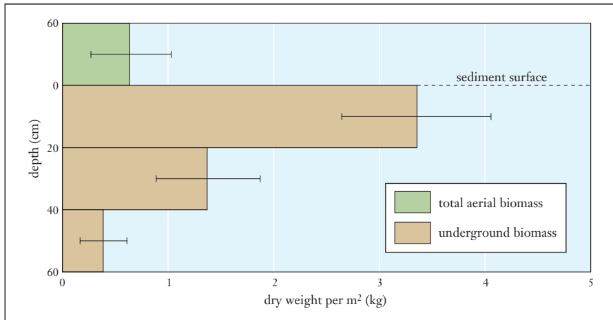
Left: The distribution of Spartina biomass on a Welsb marsh in summer. The underground system of roots and rhizomes (underground stems) far exceeds the aerial shoots in biomass, with the greatest concentration being in the top 20 cm of sediment. The plant parts in this top 20 cm are particularly vulnerable if there is subsurface penetration by light toxic oils. Horizontal bars on the figure are the statistical 95% confidence limits.
